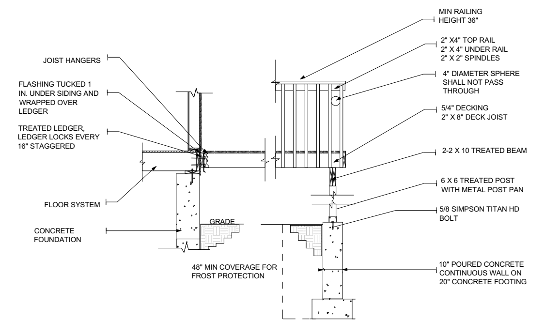
Typical Deck Detail Attached to Wood Wall
