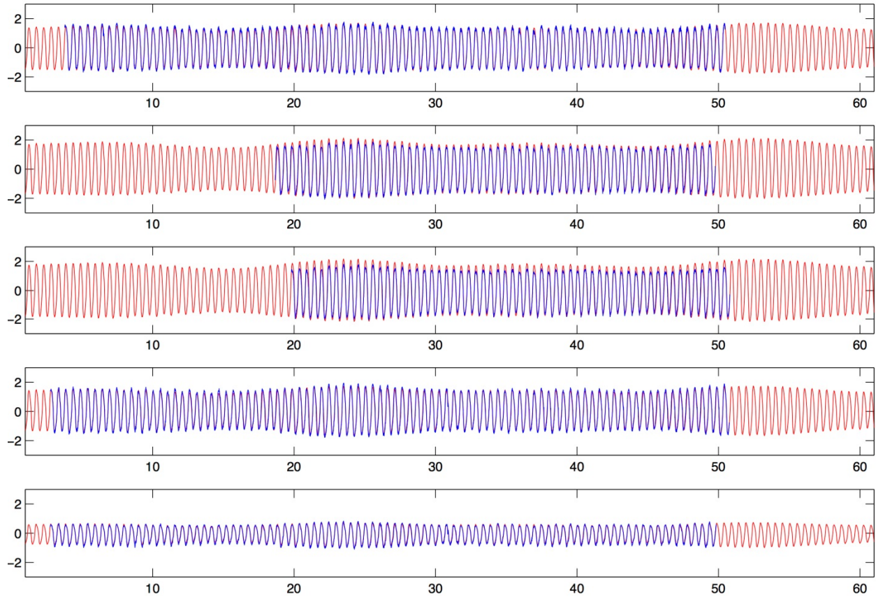
Figure 14. Comparison of time series of depth-averaged velocities ( \text{m s}^{-1} ) for the CMIST period (June-July, 2009). Time is days since June 1, 2009. The red line is the model-computed value and the blue line is the observed. The comparisons for CMIST Stations 1,2,3,5,6 (see Figure 10 for locations) are arranged from top to bottom. Note that the observations cover different time periods. Model results are shown for the first 61 days of 2009 and fully encompass each measured series.
