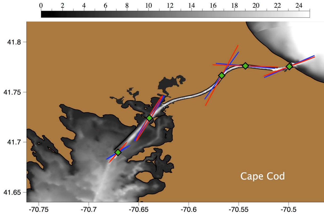
Figure 16. Tidal ellipses of model-computed (red) and observed (blue) depth-averaged velocity at CMIST stations in upper Buzzards Bay. Shading represents bathymetry (m).
