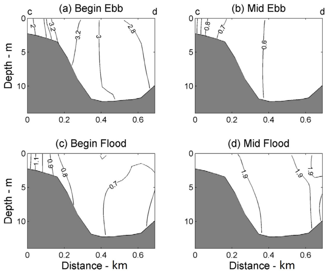
Figure 25. Same as Figure 21, except showing TN concentration fields ( \mu\text{g/l} ) in upper Buzzards Bay (along line c-d in Figure 3c).
