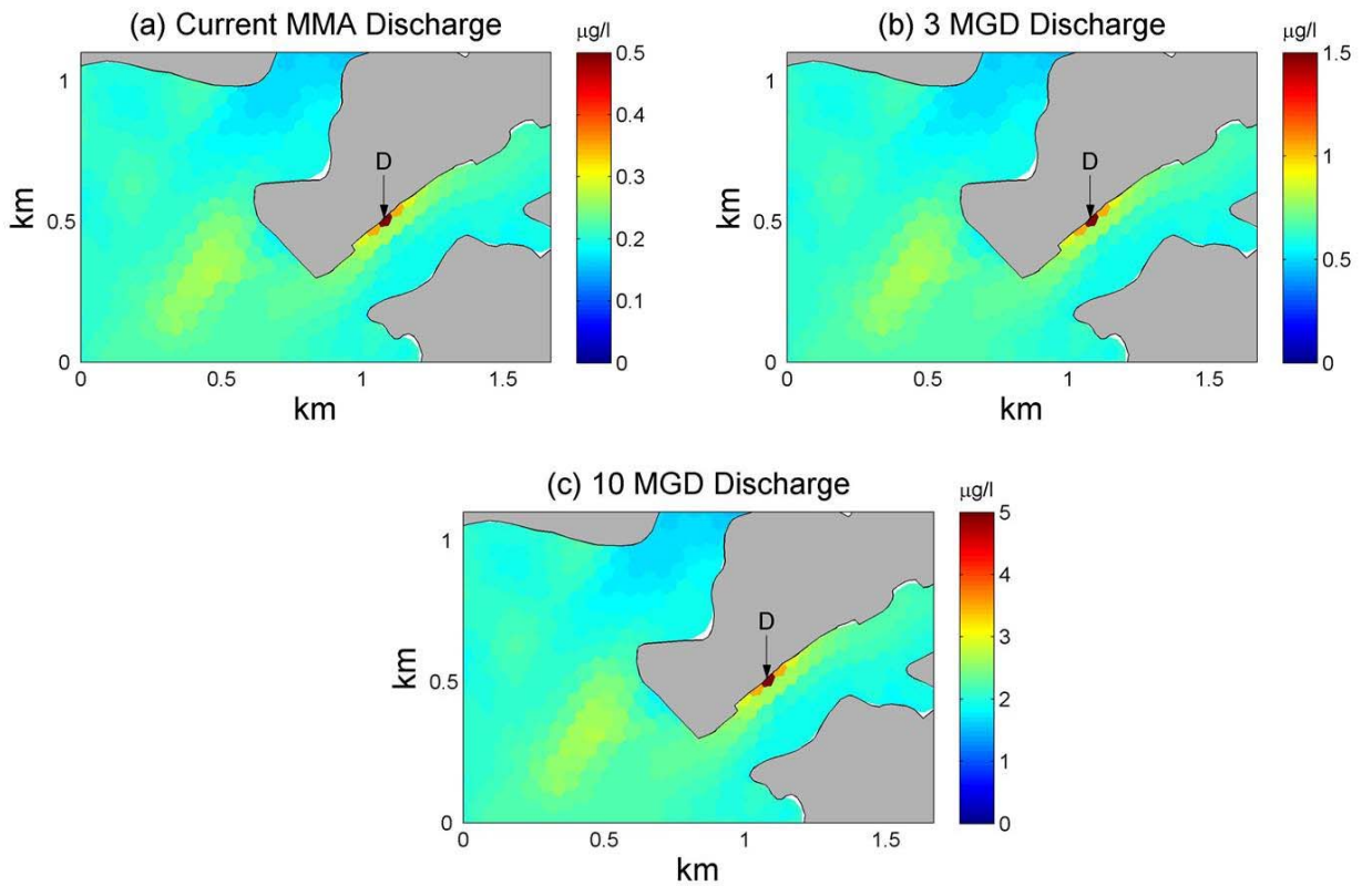
Figure 18. Vertically and temporally averaged concentrations ( \mu\text{g l}^{-1} ) of total nitrogen (TN) contained in the discharged effluent (not including the background TN concentrations) for three discharge scenarios (Table 1). The fields were computed from the model fields of July 2015. Note that different color scales are used for each panel. Note also that the maximum concentration in each panel [e.g., 7 \mu\text{g l}^{-1} in panel (c), which is slightly larger than the scale maximum to more clearly show the spatial variations of the TN field] is far lower than the background TN concentrations shown in Figures 4-5 (which are 200\text{-}800 \mu\text{g l}^{-1} ).
