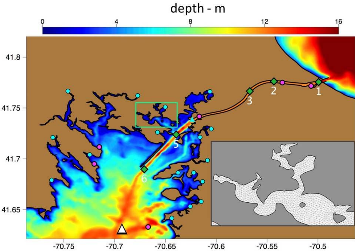
Figure 10. Portion of the FVCOM-SEMASS domain in upper Buzzards Bay with bathymetry (m) (see Figure 9 for the full model domain). Also shown are measurement locations for CMIST upward-looking ADCP (numbered green diamonds), tidal harmonic elevation stations (magenta circles), and Mass Division of Marine Fisheries long-term bottom temperature record (white triangle) as well as the locations for point sources of freshwater input to the upper bay (cyan circles) and approximate location of the proposed outfall (cyan triangle). CMIST ADCPs are numbered East to West. Lower Figure Inset: Model grid in Onset Bay.
