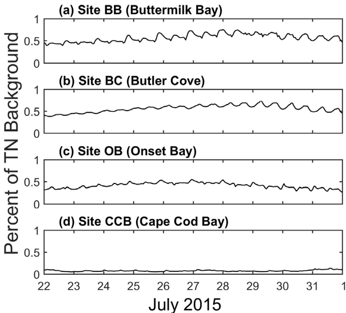
Figure 26. Same as Figure 24 except showing the effluent TN concentrations at points in each designated area (shown in Figure 3a,b) as a function of the percent of the measured TN background concentration in each area (Figure 8 and Table 2).
